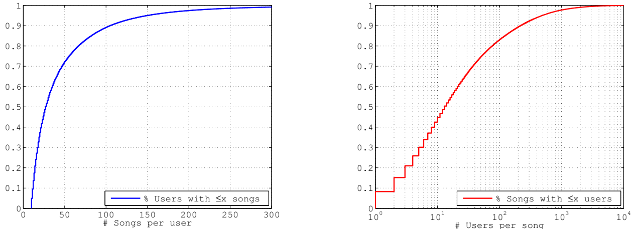
Figure 2: Left: the empirical cumulative distribution of users as a function of library size. Right: the cumulative distribution of songs as a function of number of unique users. Statistics were estimated from the training sample of 1 million users.
